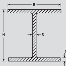
UNIVERSAL COLUMN
