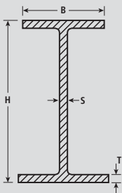
UNIVERSAL BEAM
